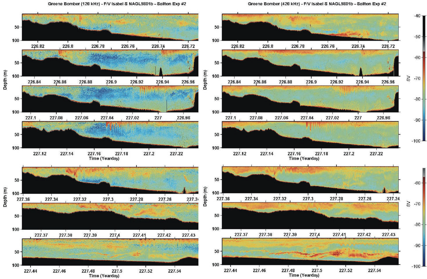
Figure 7. The second acoustic survey transect between Scituate, Massachusetts and Stellwagen Bank. Left and right panels illustrate scattering at 120 kHz and 420 kHz, respectively. The survey began slightly to the west of Stellwagen Bank in the top panel and the ship moved from east to west (right to left).
